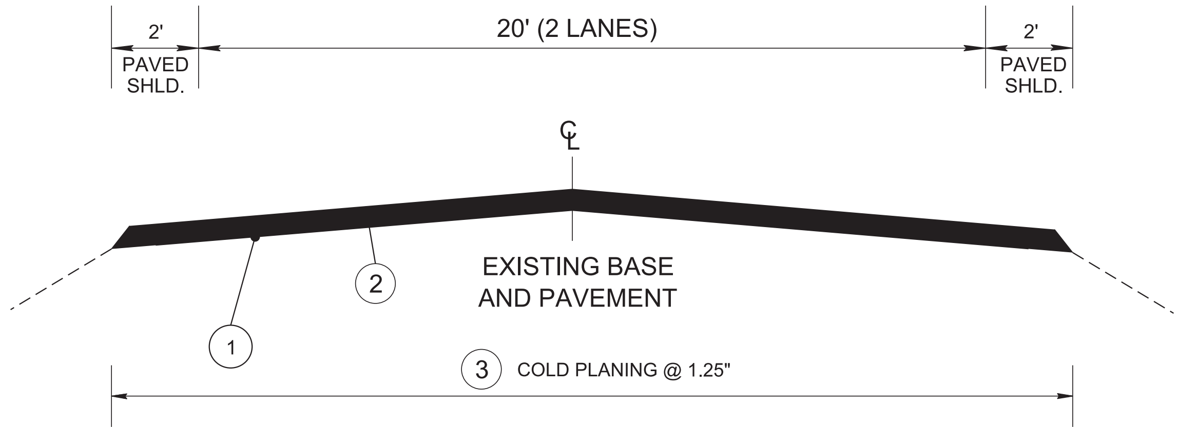
DAVIDSON COUNTY SR-251 TYPICAL SECTION
